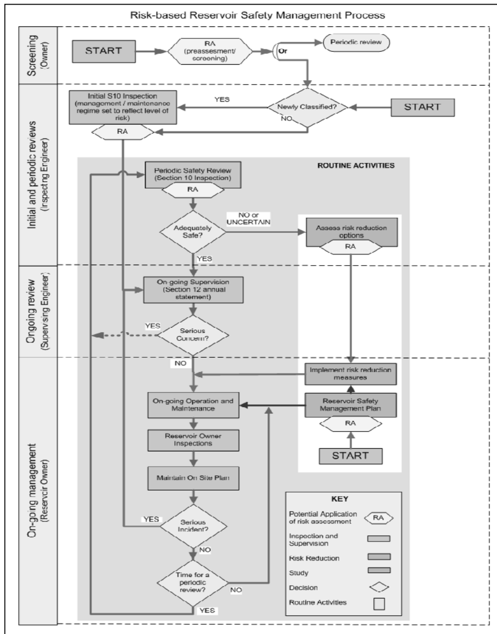
Figure 1. UK reservoir safety management process illustrating the potential role of risk assessment in decision making
