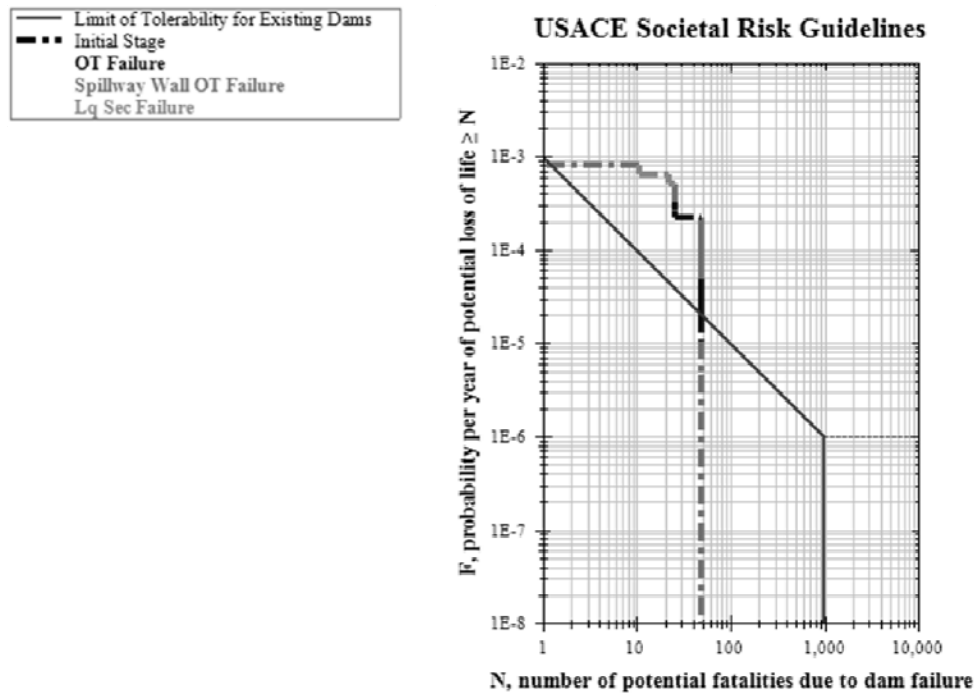
Figure 4. Example analysis for societal risk against USACE guidelines (from DAMRAE)
